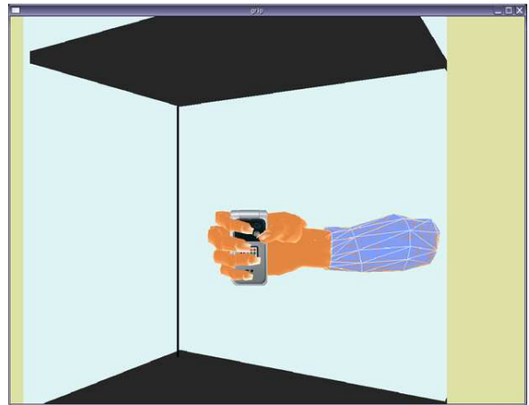
Figure 8. Execution screen
